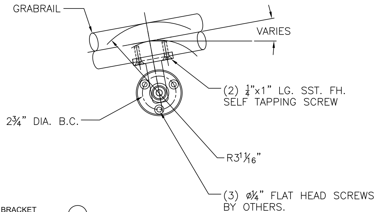
#88 ARCHITECTURAL BRACKET WALL MOUNTING (VARIABLE SLOPE) (100)
